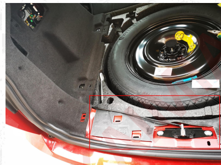
7、 Remove the original car lock, then install our lock hook. The lock driver is placed in the trim panel on the left side of the trunk.
