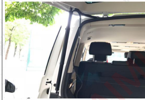
7. Install left and right electric struts, with the outlet end facing the tailgate.
