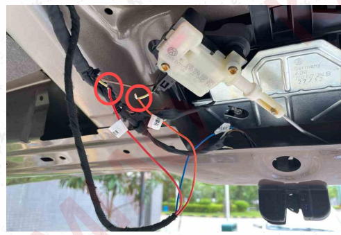
14. Cut the milky white wire, and then connect our orange lock power output wire to this end. Connect the red lock input wire to the other end.
