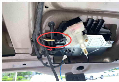
13. Unplug the 2 pin socket of the tailgate lock.
