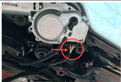
17. As shown by the arrow, the ground wire is connected to the brown ground wire of the original car's wiper motor plug.
