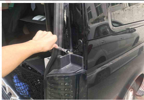
5. Remove the vehicle body ball head and install our ball head.
