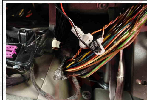
23. Remove the middle of the bottom cover under the steering wheel and find the twisted pair wiring harness as shown in the picture (black CAN-H connects to the original orange-black wire, orange CAN-L connects to the original orange-brown wire).
