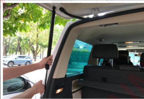
4. Remove the left and right poles of the original car.
