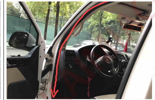
22. The power cord is passed along the original car roof to under the main driver's seat.
