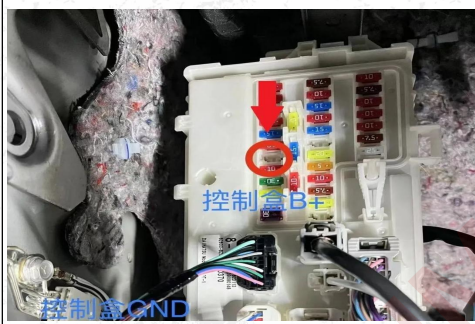
4. Take power from the driver's fuse box.
