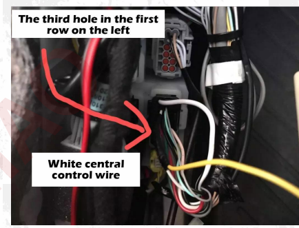
9. Connect to the central control wire at B-Pillar.
